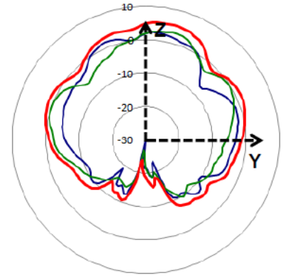
YZ-cut
