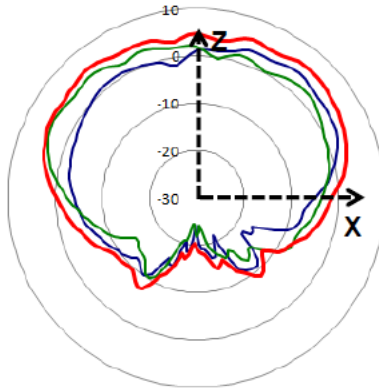
XZ-cut
